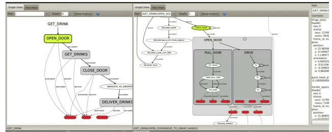
Fig. 7. Multiple levels of the SMACH plan for the Drinks Application as rendered by the SMACH Viewer . Left: The top level of the hierarchy, showing the robot actively opening the door as designated by the highlighted OPEN_DOOR node. Right: The mutually-preempting concurrence and state machines involved in opening the door, another level deeper into the SMACH plan tree.
