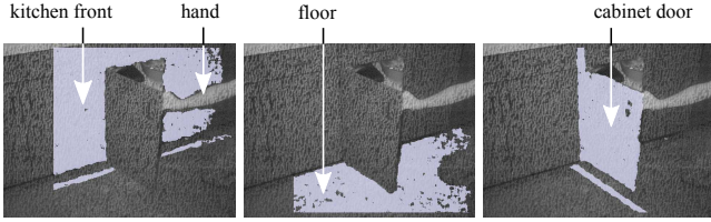
Fig. 3. Finding the three most prominent planes with our RANSAC-based approach.
