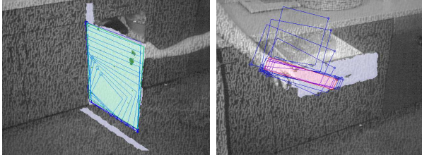
Fig. 5. Left: In each plane, we pick a random starting point from which we optimize iterative the pose and size of the candidate rectangle. Right: As our model fitting procedure is greedy, it can get trapped into local maxima.
