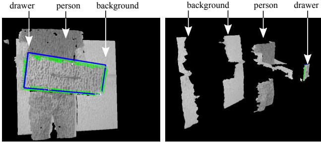
Fig. 8. The blue rectangle shows the ground truth location obtained with a motion capturing studio, while the green rectangles show our estimates.
