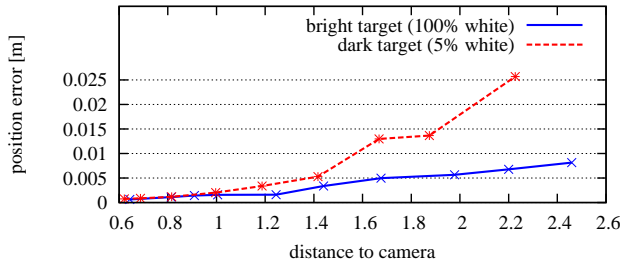
Fig. 2. Positional error of a planar target, observed with our active stereo system. For a white target, the error stays below 2mm until after 1.2m, then goes up to about 1cm at 2.5m. For a very dark target, error is low close up, then becomes larger at distance, when the pattern is difficult to see.
