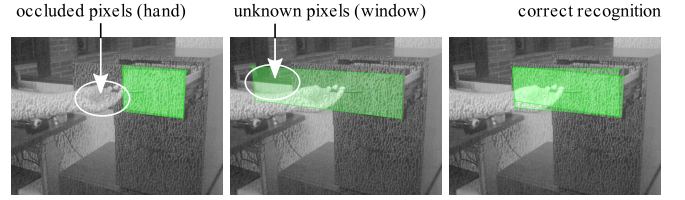
Fig. 4. Effect of the cost parameter for unknown and occluded pixels. Left: cost too high (1.0). Middle: cost too low (0.0). Right: good (0.2).
