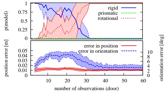
Fig. 9. Evaluation of the articulation models learned for a cabinet door, averaged over 50 runs. The plots at the top show the probability of the articulation model templates, the plots at the bottom show the prediction error of the learned model.
